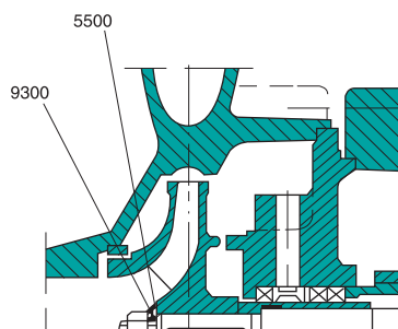
Impeller unbalanced
