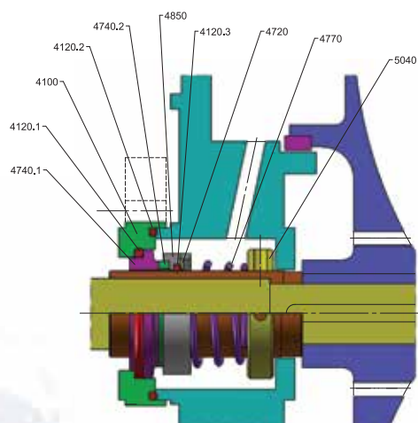
Single Mechanical Seal
