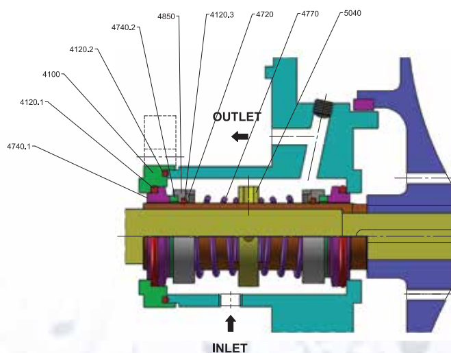
Double Mechanical Seal
