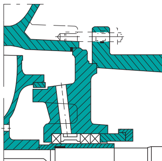
"Push-in" discharge cover
